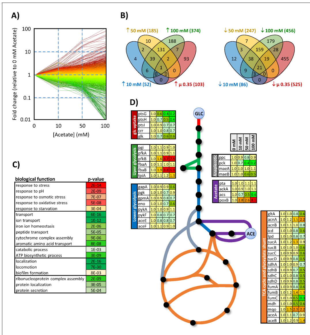
Figure 2. Response of the E. coli transcriptome to changes in acetate concentration (0, 10, 50, or 100 mM) during growth on glucose (15 mM). The changes in gene expression are shown in (A). Each line represents the expression of a single gene relative to its expression level measured in the absence of acetate. Up- and downregulated genes are shown in red and green, respectively. The Venn diagrams (B) represent the total number of genes upregulated (left) and downregulated (right) by at least a factor of 2 under each condition and during growth on glucose in the absence of acetate but at the same growth rate as in the presence of 100 mM acetate ( 0.35 \text{ hr}^{-1} , extrapolated from the data from Esquerré et al., 2014 ). Biological functions modulated by the presence of acetate (based on Gene Ontology analysis) are shown in (C), with the corresponding p-values. The expression levels of central metabolic genes are shown in (D). The data were obtained from four independent biological replicates for each condition. The online version of this article includes the following source data for figure 2:
