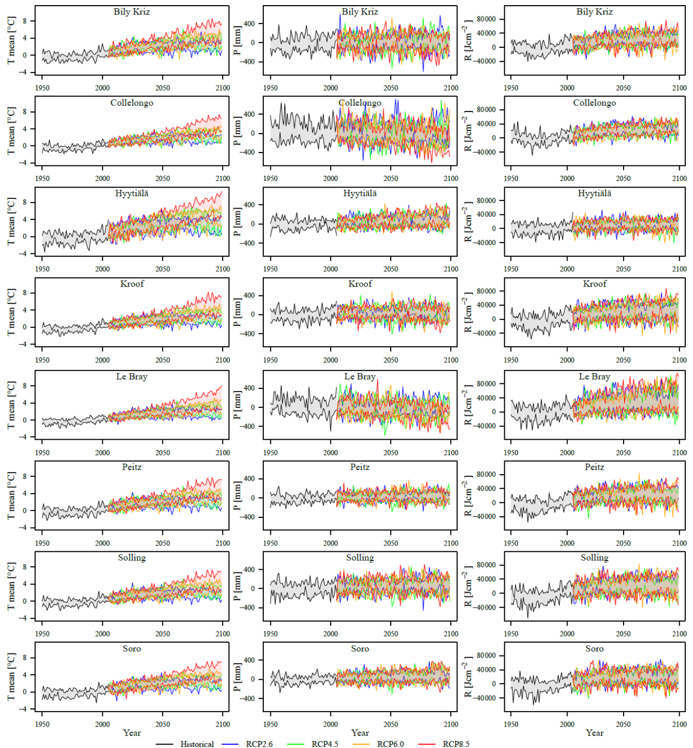
Figure 2. Change in mean annual temperature ( T_{\text{mean}} ), annual precipitation sum ( P ) and annual sum of global radiation ( R ) over the time period 1950–2099 relative to the 1980–2005 average for the ISIMIPFT scenarios. Please note that the two Solling sites have the same climate.
