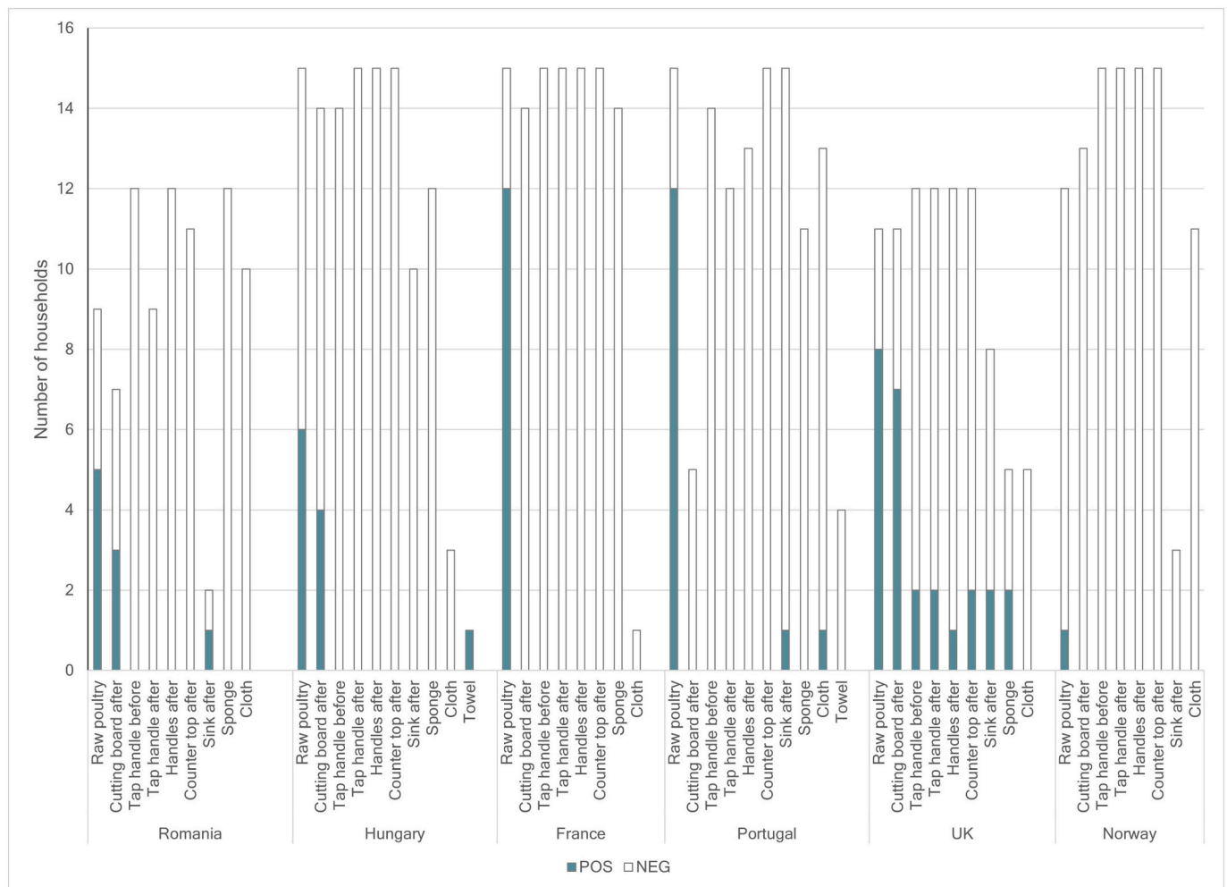
Fig. 1. Campylobacter positive samples in blue and negative in white from 87 kitchens, from sites sampled before and after food preparation. In addition to the samples shown, which included all Campylobacter -positive sample types, 145 samples that were all negative for Campylobacter were taken before food preparation from cutting board, countertop, handles, sink, or refrigerator. (For interpretation of the references to colour in this figure legend, the reader is referred to the web version of this article.)
