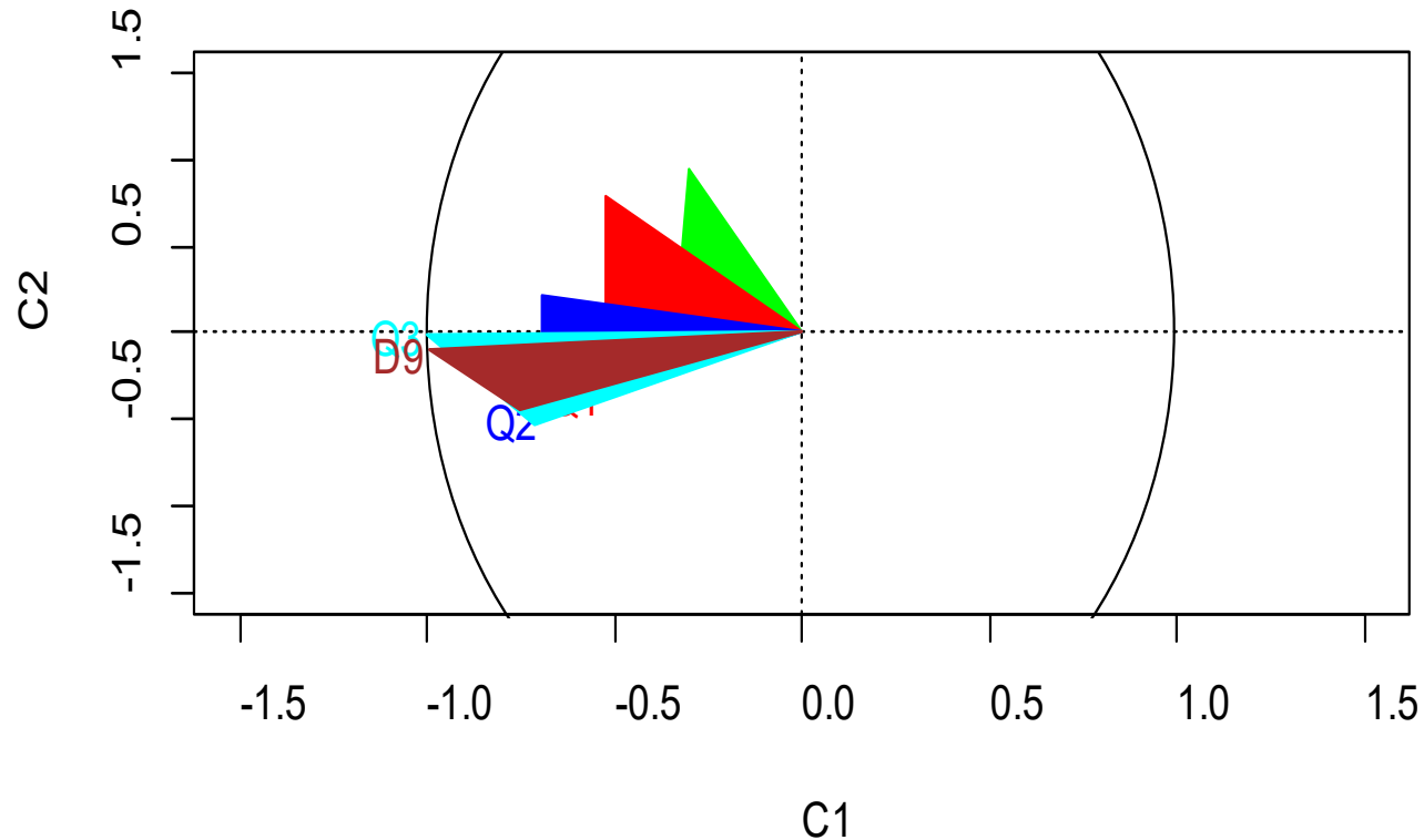
Correlation Circle
