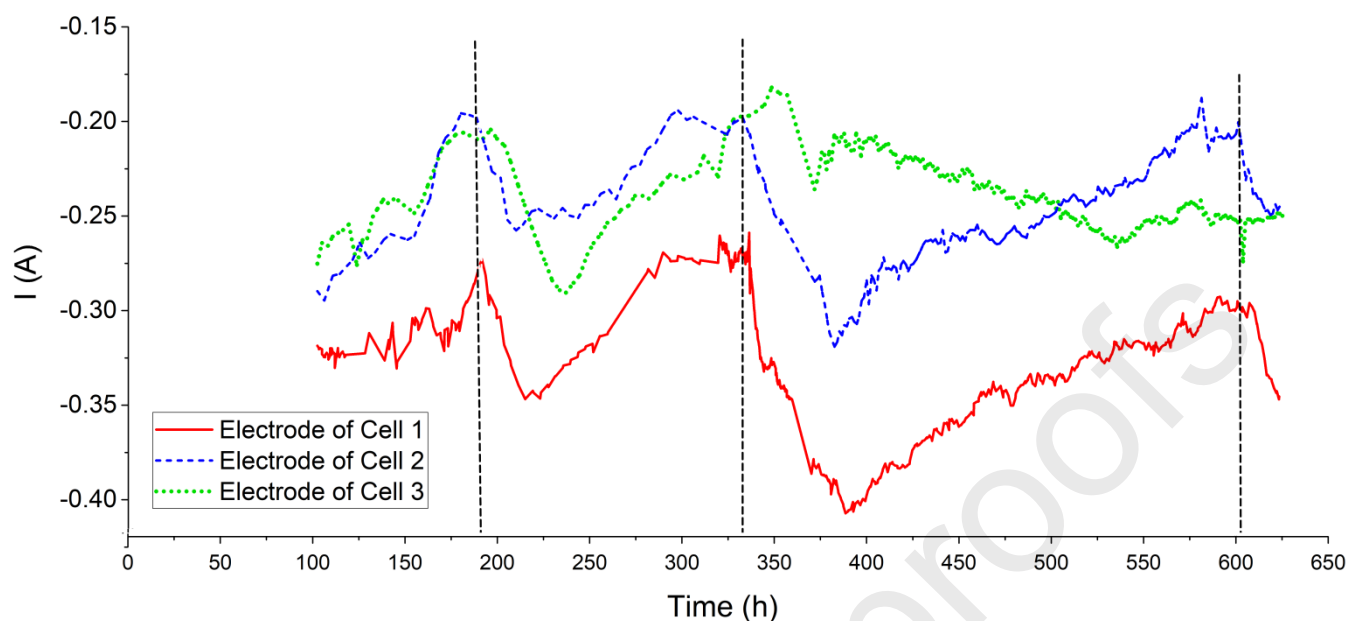
Figure 2. Current vs. time evolution at the electrodes incubated in the pilots 1, 2 and 3. The potential was set at - 0.5 V vs. SCE from day 4 to the end of the experiment at day 26 (623 h). The initial concentration of nitrate was set at 400 mg.L -1 . Three more sodium nitrate additions (500 mg.L -1 of NO 3 - each) were made in each pilot during the course of the experiment (namely at 190 h, 336 h and 600 h).
