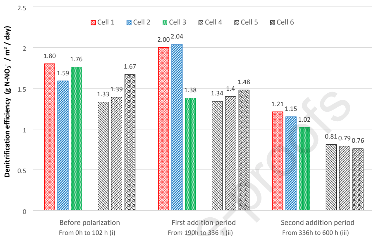
Figure 3: Nitrate removal efficiency on the three periods of the experiment in g of \text{N-NO}_3^- removed per day and \text{m}^2 of sediments (the surface for each pilot was 44.15 \text{ cm}^2 ). The total experiment time was divided in three different periods: (i) before polarization, (ii) between first and second sodium nitrate addition and (iii) between second and third sodium nitrate addition.
