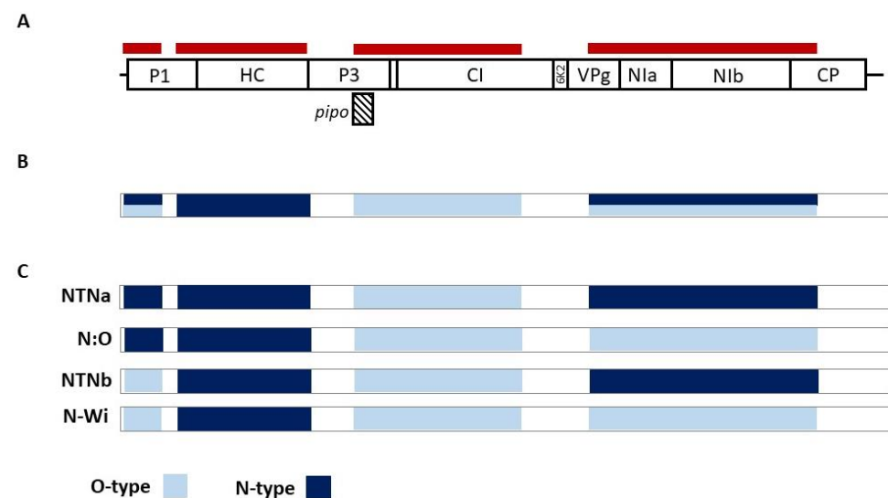
Figure 2. Analysis of samples showing multiple infections by PVY strains. (A) Schematic representation of the positions of informative regions (red stripes) along the PVY genome used for PVY-O- and N-specific mapping of HTS reads (B) Graphical representation of obtained sequences from samples T1, T40, and T62, where positions with more than one variant detected are shown (azure/dark blue) (C) Possible recombination patterns of PVY variants present in T1, T40, and T62 samples.
