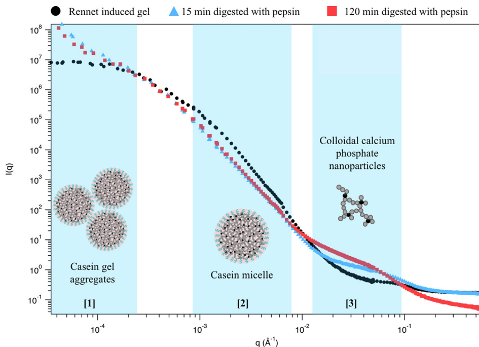
Fig. 6. Schematic representation of the models applied to segments of a combined small angle neutron scattering (SANS) and ultra-small angle neutron scattering (USANS) curve at different size scales used for the present study. The example provided is a rennet-induced gel (RG) and its digesta prepared and digested in H 2 O after 15 and 120 min.
