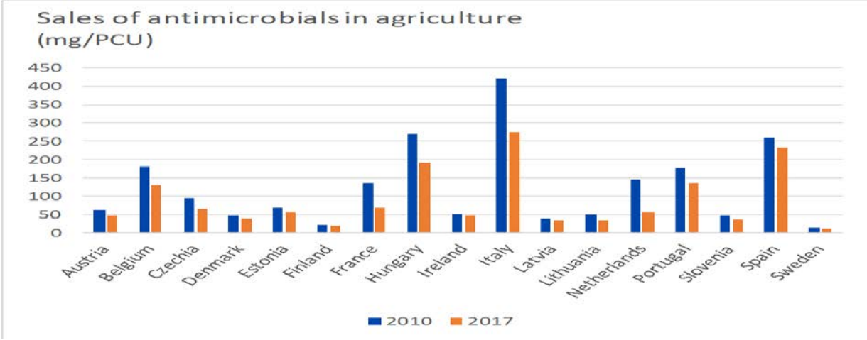
Figure 3.9: Sales of antimicrobials in agriculture in various MS, in mg/PCU, in 2010 and 2017
