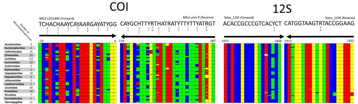
FIGURE 1 In silico evaluation of COI and 12S primers. Base composition plots (green = thymine, blue = cytosine, red = adenine, yellow = guanine) generated with PrimerMiner for the MG2-COI and 12S-Teleo primer binding sequences. For each fish family present in the study area, sequences were extracted from complete mitochondrial genomes downloaded from NCBI (and BOLD for COI). The COI and 12S primer positions are relative to the Folmer region (Folmer et al., 1994) and the Cyprinus Carpio mitochondrial genome (Valentini et al., 2016), respectively
