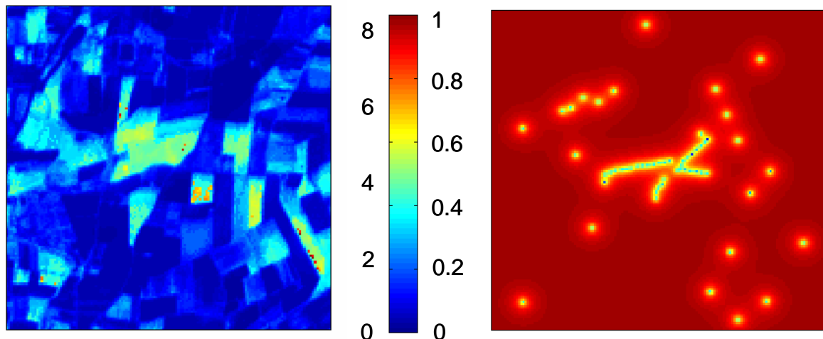
Figure 10. Co-located kriging applied to the Alpillles site (2001). The figure on the left represents the estimated LAI map. That on the right represents the weight \delta associated to the radiometric information from the high spatial resolution image. The ESUs are associated to the lowest values of weights \delta . The lowest values of the weights \delta are located near ESUs. Note that for this site, two transects of ESUs were sampled in the middle of the site.
