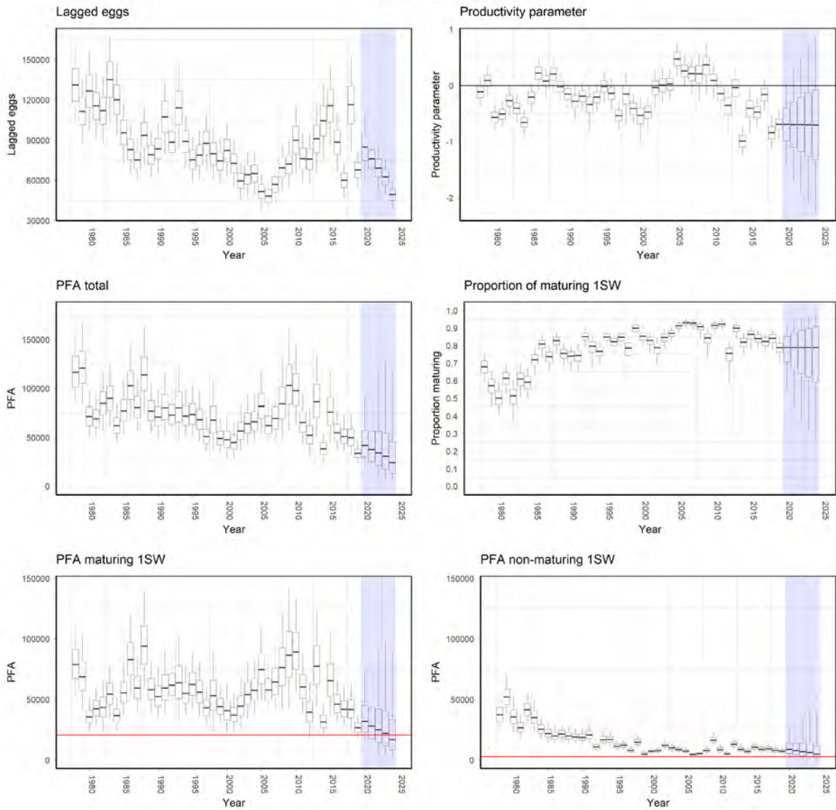
Figure 3.4.3.6. Iceland (south/west regions): Lagged eggs (in 1000s) from 1SW and MSW spawners combined, productivity parameter from eggs to PFA, total PFA, proportion 1SW maturing, and PFA of maturing and non-maturing stocks, for PFA years 1978 to 2024. For PFAs, proportion maturing and productivity parameter for the last five years (2020 to 2024) are forecasts (as indicated by the blue shaded region). The horizontal lines in the bottom panels are the age-specific SER values. Box and whiskers show the 5th, 25th, 50th, 75th and 95th Bayesian credible intervals (BCIs).
