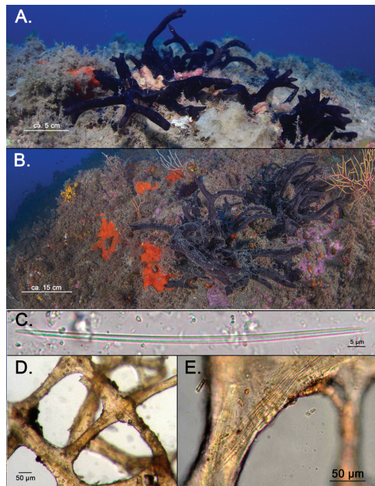
Fig. 2: A and B) Individuals of Chalimula nigra growing onto rocky coralligenous substrates in el 'Tajo del Pirata', partially covered by an algal turf. Scale bars are approximate. C) Detail of the oxneas as seen on an optical microscope; scale 5 µm. D) Spongin fibers in a ladder-like reticulation, with primary and secondary fibers undistinguishable; scale 50 µm. E) Detail of the spongin fibers, where several oxnea can be seen forming the tracts of the skeleton; scale 50 µm.
