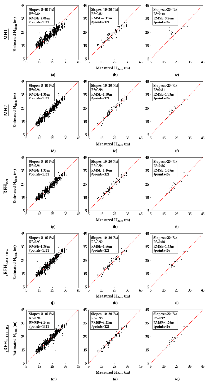
Figure 7. Comparison of the measured vs. estimated dominant height from the models presented in Section 3.1 (Table 2) using GEDI metrics extracted with the processing configuration “a1” of GEDI data.
