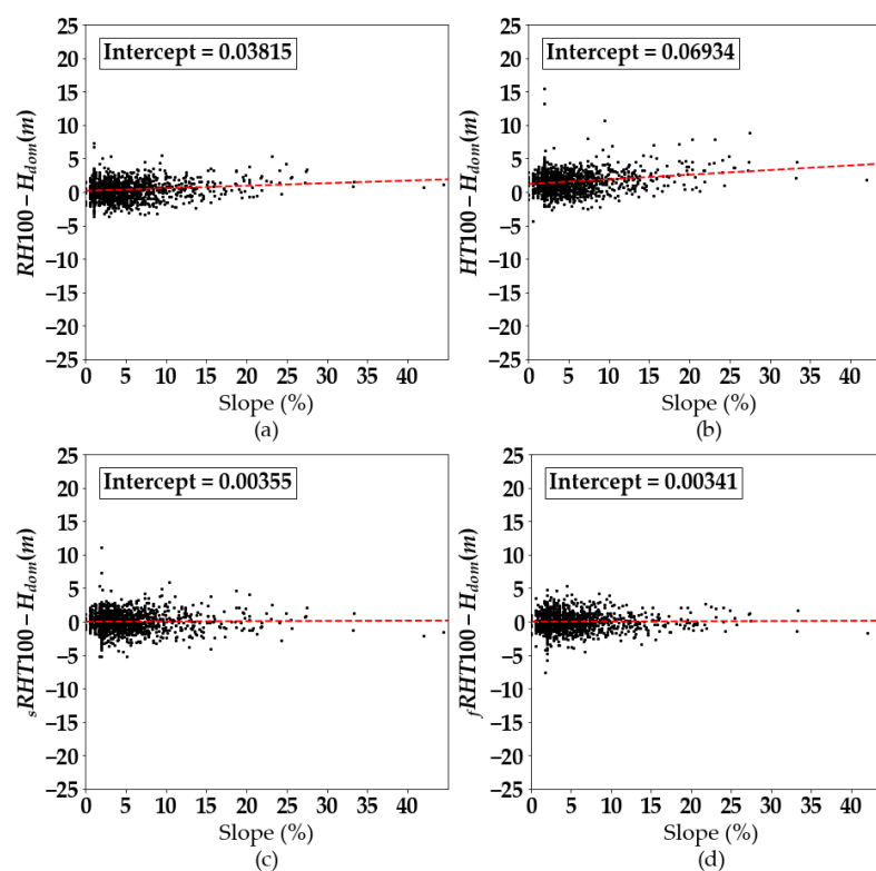
Figure 11. Distribution of several GEDI metric height errors by slope gradient.
