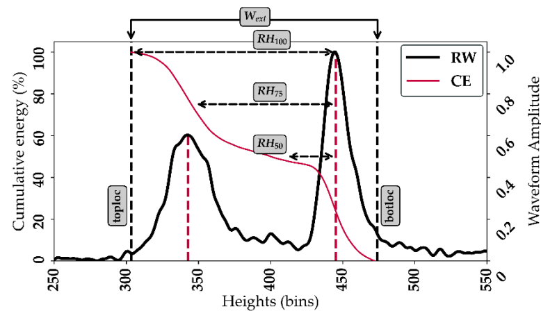
Figure 2. Example of an acquired GEDI waveform (RW) over an Eucalyptus stand ( H_{dom} = 20.4 m; V = 129.6 m 3 ·ha -1 ). The cumulative energy of the waveform (CE) between botloc and toploc and the corresponding relative heights ( RH_n ) at different quantiles “ n ”. The left and right red dashed lines represent, respectively, the position of the vegetation ( Vloc ) and ground peaks ( Gloc ). Note that 1 ns corresponds to 15 cm sampling distance in the waveform. The waveform amplitudes are counts from the analog to digital converter (ADC) on the instrument and normalized to be between 0 and 1.
