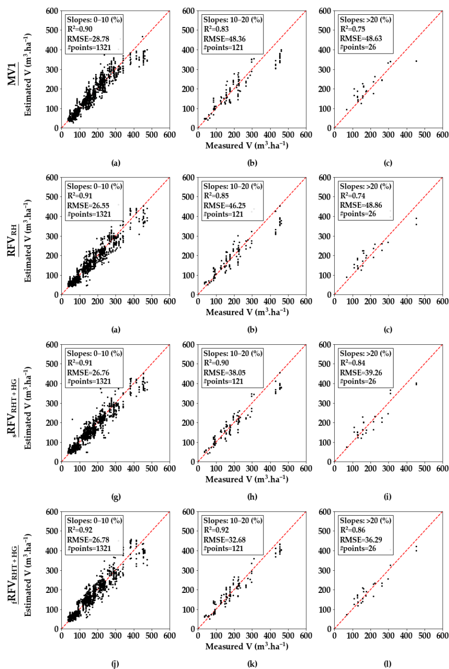
Figure 9. Comparison of measured vs. estimated wood volume from the models presented in Section 3.2 using GEDI metrics extracted using algorithm a1. RMSE is expressed in m 3 ·ha -1 .
