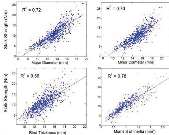
Figure 3: Linear regression and coefficient of determination ( R^2 ) value between stalk strength and various geometric features.
