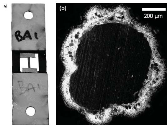
Fig. 1 : a) Specimen mounted in laser-cut cardboard frame for tensile testing. Retroflective tapes are used for laser extensometry. b) Cross-section area of the stems was determined using optical microscopy.
