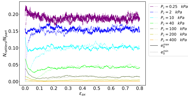
Figure 7. Proportion of rattlers in S2 simulations
