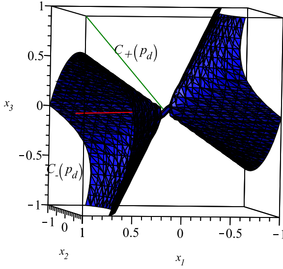
Figure 5. Isotropic cone (blue surface) for the load p_d = (\frac{3}{2}, \frac{3}{2}) of the three degree of freedom discrete Leipholz column: \det K_s(p_d) < 0 . Outside the isotropic cone (for example in the green line direction), then X \in C_+(p_d) : X^T K_s(p_d) X > 0 . Inside the isotropic cone (for example in the red direction), then X \in C_-(p_d) : X^T K_s(p_d) X < 0 . On the isotropic cone (blue surface), X^T K_s(p_d) X = 0 .
