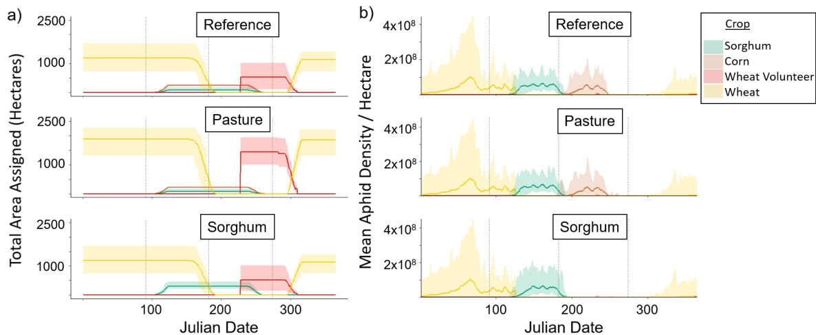
Fig. 2. Area assigned (a) and mean aphid density per hectare (b) throughout the year for each simulated crop type. Bold lines represent the mean values across all simulations, and the shaded areas represent minimum and maximum value ranges. Each plot represents a different scenario with the reference scenario on top, the pasture scenario where all pastures are replaced by wheat within the rotations in the middle, and the sorghum scenario where corn is replaced by sorghum within the rotations on the bottom.
