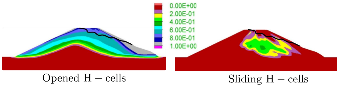
Figure 16. Proportions of the H-cells in which contact has been lost ( f_{open} , left) or sliding has occurred ( f_{slide} , right) at failure ( H_w = H_r and t = 1.3 s). The black solid line corresponds to the piezometric level.
