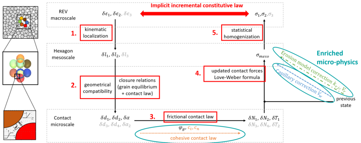
Figure 3. Five steps homogenization scheme of the H-model. Additional variables for the three-dimensional case are shown in grey. Current developments on the enriched versions of the model are highlighted.
