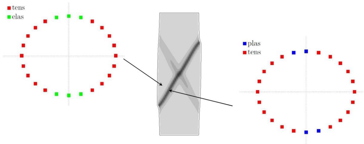
Figure 9. Directional analysis of the contact regimes of hexagons outside (left) and inside (inside) the shear band ( \epsilon_1 = 0.08 ).
