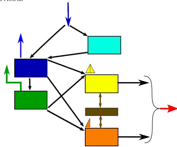
(f) GR4J-CemaNeige of airGR, modified from de Boer-Euser et al. (2017).
