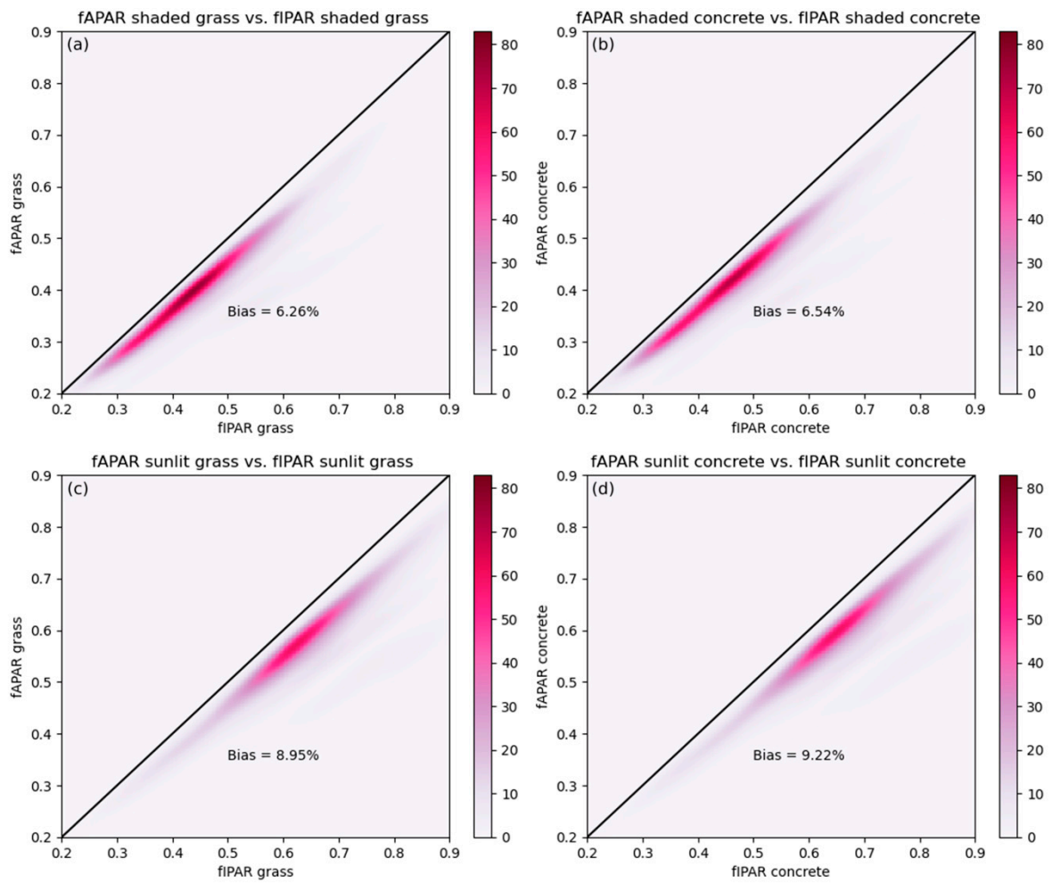
Figure 6. The juxtaposition of the fAPAR and fIPAR values at different backgrounds (grass (a,c) and concrete (b,d)) and illumination conditions (sunlit and shaded leaves). The legend represents the density of points.
