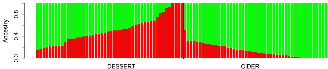
Figure 3 Population structure of 96 apple cultivars from the cider and dessert genetic pools. Membership probabilities were obtained with ADMIXTURE for K = 2 . The bar plot, generated using the qqman package in R, shows each individual as a vertical bar.
