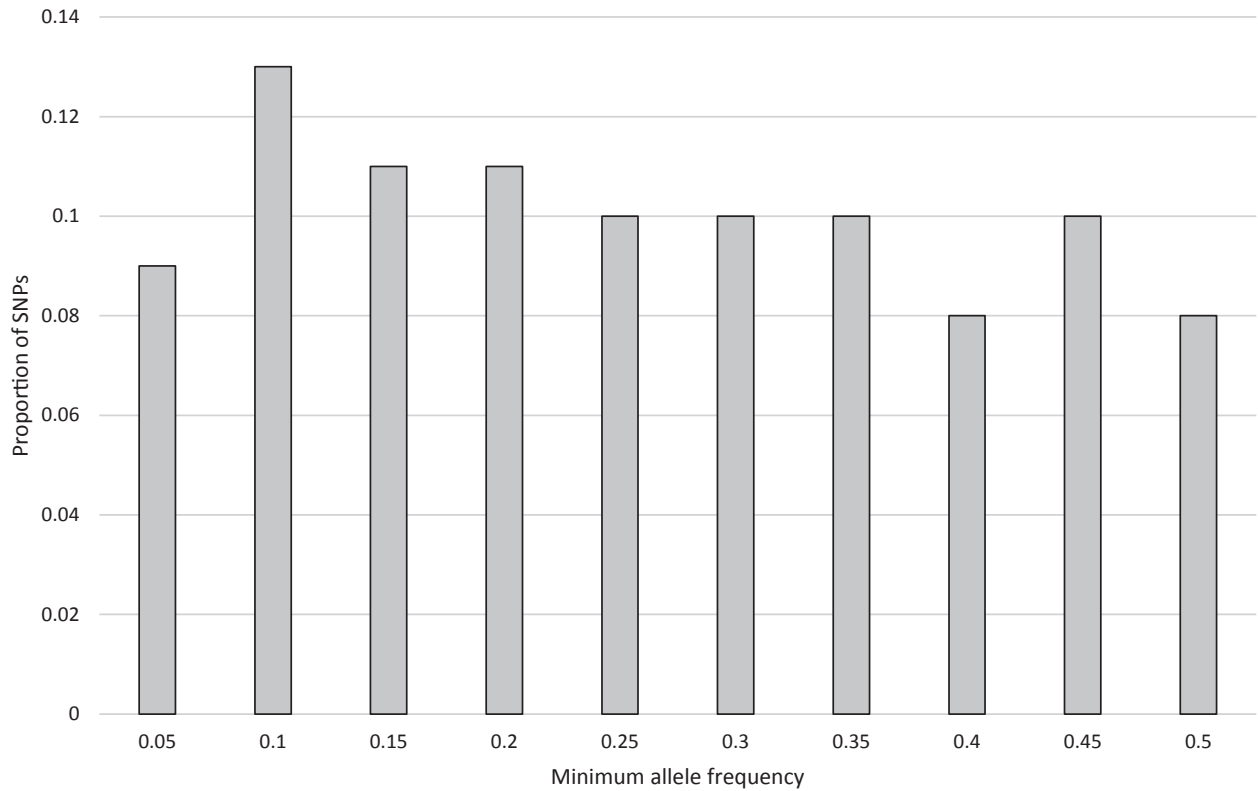
Figure 1 Allele frequency spectrum of the 3704 SNP markers of the array.
