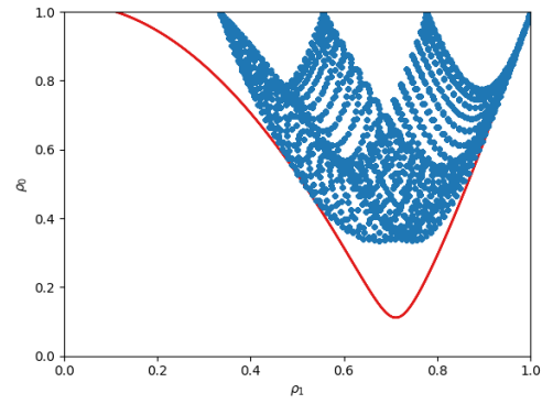
(b) Lamination points and envelope, n_1 = 1 , n_2 = 2 , n_3 = 6
