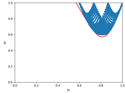
(d) Lamination points and envelope, n_1 = 1 , n_2 = 2 , n_3 = 12
