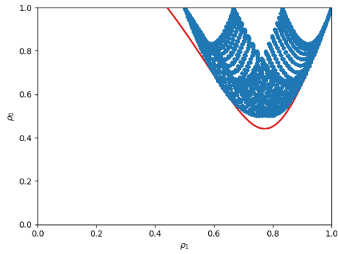
(c) Lamination points and envelope, n_1 = 1 , n_2 = 2 , n_3 = 9
