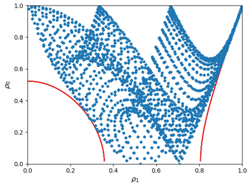
(a) Lamination points and envelope, n_1 = 1 , n_2 = 2 , n_3 = 3
