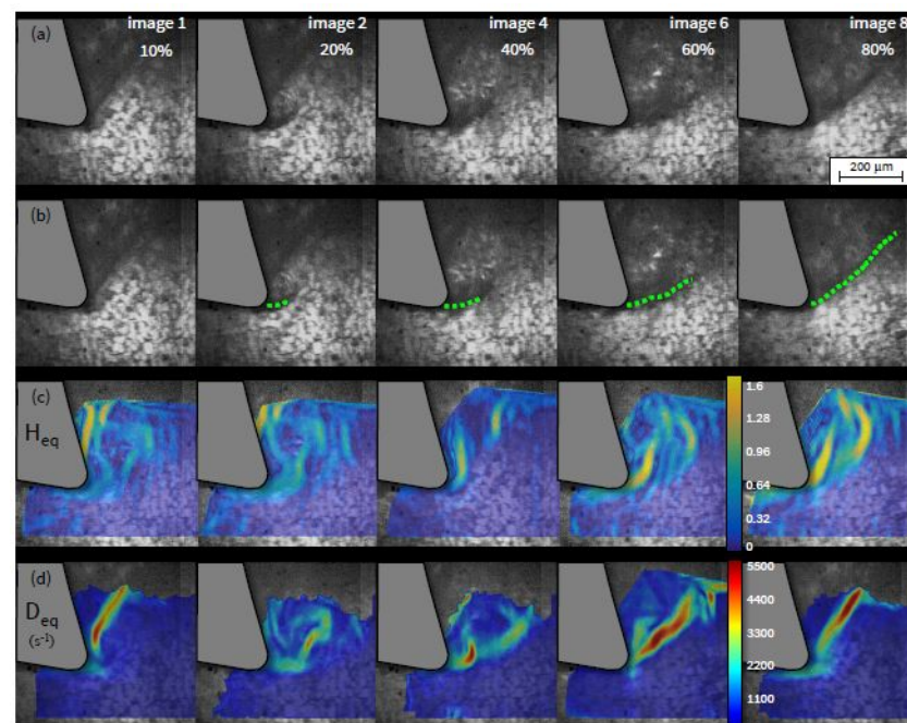
Figure 14. (a) Captured visual images at different instants during one segment chip formation; (b) crack propagation within the PSZ; and, (c) cumulative Henky strain field and (d) the equivalent strain rate field [49].
