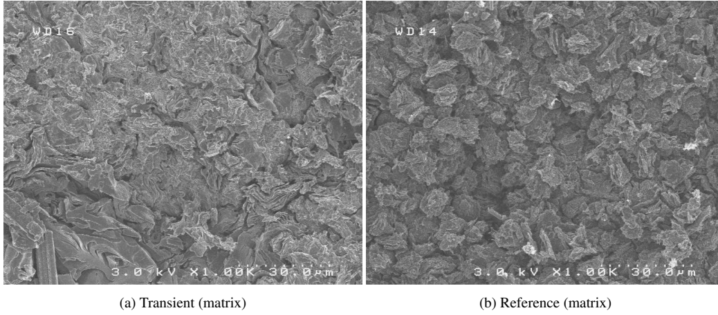
Figure 11: SEM micrographs of the matrix after 15 s and 30 s of exposure to a 10 \text{ MW m}^{-2} heat flux. Other experimental conditions are given in table 1 for Transient and Reference tests, respectively.
