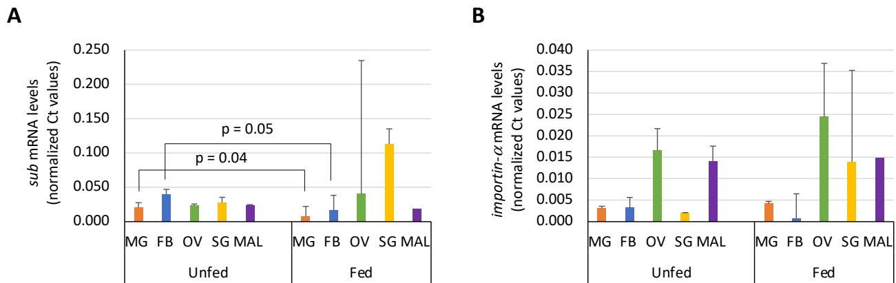
Figure 3. Expression profile of sub and importin- \alpha in Ixodes ricinus organs. The mRNA levels of (A) sub and (B) importin- \alpha were determined by qRT-PCR in unfed and fed female I. ricinus midgut (MG), fat body (FB), ovary (OV), salivary glands (SG) and Malpighian tubules (MAL). The Ct values were normalized against tick elongation factor (average + S.D.) and compared between fed and unfed ticks by Student's t-Test ( p < 0.05 ; 3 biological replicates with 7–10 ticks per replicate).
