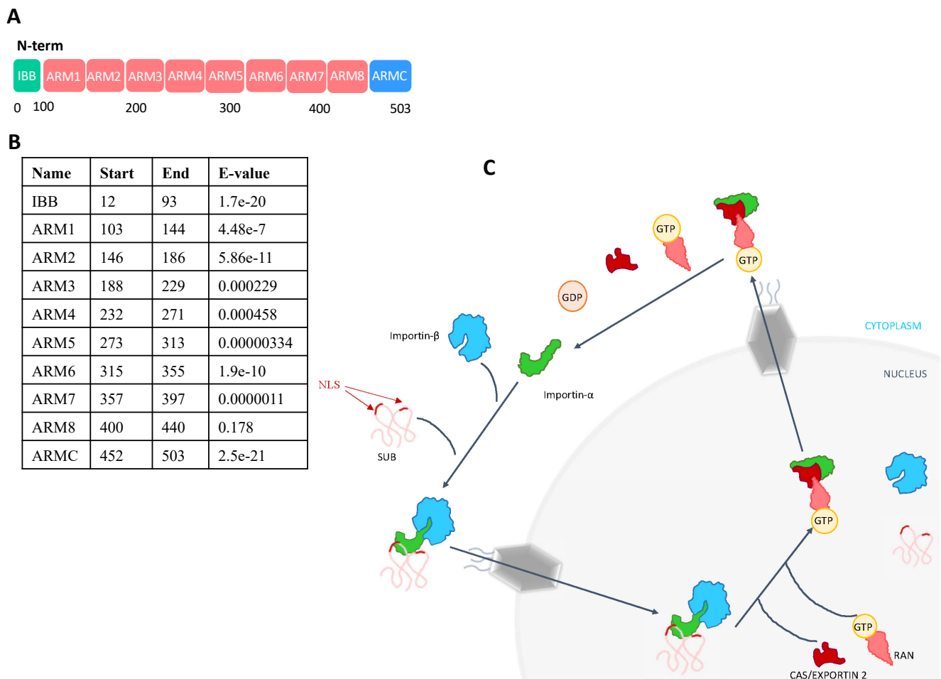
Figure 2. Protein domain architecture analysis and transport cycle of Importin- \alpha . (A) Graphical representation of the predicted protein domains of tick Importin- \alpha . These include an Importin- \beta binding domain (IBB), eight Armadillo/beta-catenin-like repeats (ARM 1-8) and an atypical ARM repeat in the C-terminal region (ARMC). (B) Confidence (E-value) of the predicted tick Importin- \alpha domains and repeats. The analysis and the prediction were carried out using the SMART tool ( http://smart.embl-heidelberg.de/ , accessed on 12 October 2020). (C) Importin- \alpha binds to NLS-cargo proteins such as SUB and also to Importin- \beta . Importin- \beta / \alpha -SUB could be translocated into the nucleus by the interaction with the nuclear pore complexes. Then, proteins such as Exportin-2 and Ran-GTP trigger the dissociation of the Importin- \beta / \alpha -SUB complex through binding to Importin- \alpha . Finally, Importin- \alpha is recycled to the cytoplasm.
