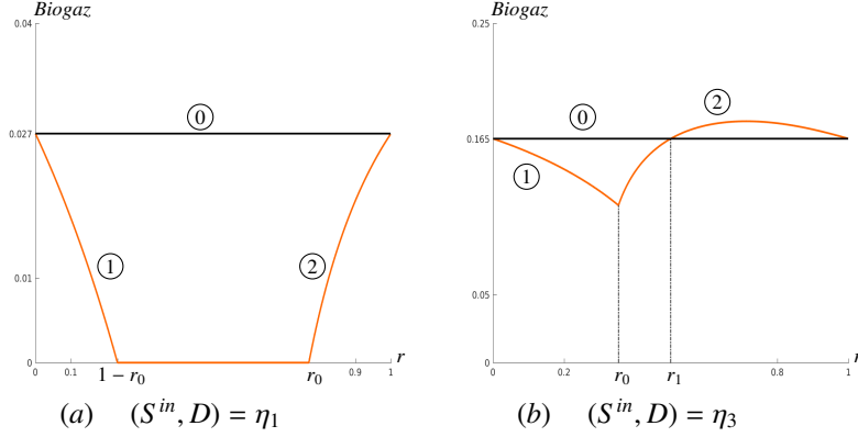
FIGURE 9. The biogas flow rate of the serial configuration with respect to r \in [0, 1] , corresponding to points \eta_1 and \eta_3 depicted in Figure 8. The numbered curves ① (in black), and ①, ② (in orange) are respectively defined by y = G_{chem}(S^{in}, D) , y = G_1(S^{in}, D, r) and y = G_2(S^{in}, D, r) . Recall that r_0 = D/(f(S^{in}) - a) and r = r_1 is the solution of S^{in} = g_r(D) . In (a): (S^{in}, D) = \eta_1 and r_0 \approx 0.77 . In (b): (S^{in}, D) = \eta_3 , r_0 \approx 0.35 and r_1(0.5, 0.6) = 0.5 .
