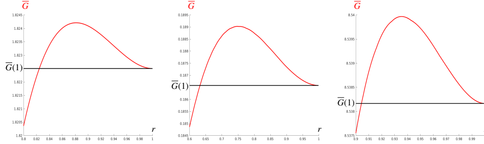
FIGURE 15. The map r \mapsto \bar{G}(r) with \bar{G} defined by (4.24). In (a): f(S) = 4S , a = 0.6 and S^{in} = 1.5 . In (b): f(S) = 4S/(5+S) , a = 0.3 and S^{in} = 1.5 . In (c): f(S) = 4S^2/(25+S^2) , a = 0.3 and S^{in} = 10 .
