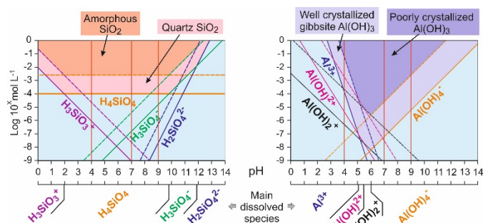
Fig. 6 Dissolved species concentration at equilibrium and precipitation domains in aqueous solution for Si (left) and Al (right) at 25°C. Calculation was done using the MINTeq database values. 18 Plain lines: species at equilibrium with well crystallized minerals; dashed lines: species at equilibrium with poorly crystallized or amorphous minerals. Vertical red plain lines mark the studied pHs.
