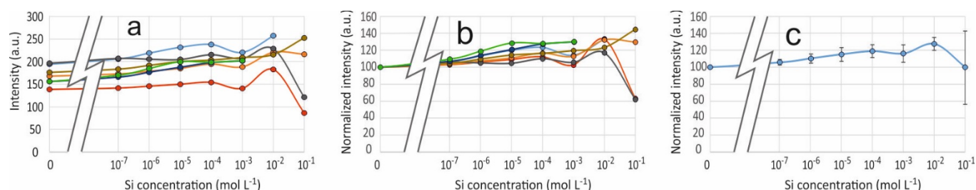
Fig. 2 Intensity of the 510 nm emission peak at \lambda_{\text{ex}} = 330 nm for the PDMPO-Si system at pH 4 (7 measurements). a: bulk values; b: values normalized to the PDMPO only value; c: average and standard deviation given by the vertical bars.
