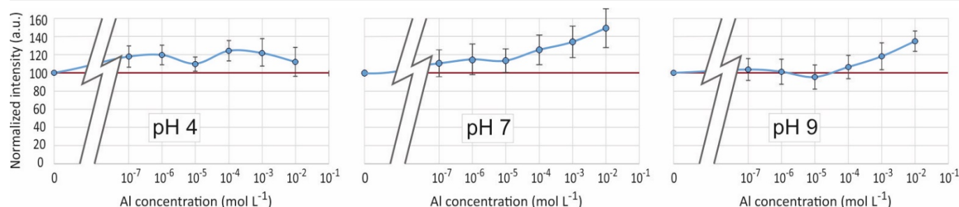
Fig. 8 Fluorescence intensity at \lambda_{ex} = 330 nm, \lambda_{em} = 510 nm of the PDMPO-Al system at various pH as a function of the concentration of Al in mol L -1 .
