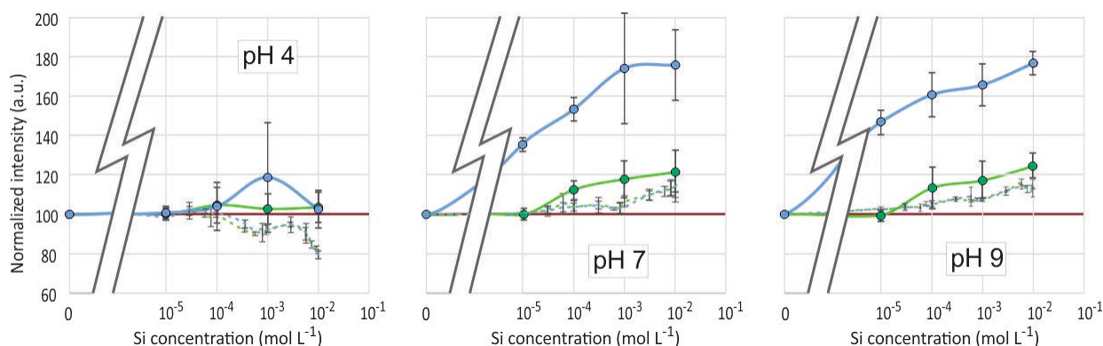
Fig. 12 Fluorescence intensities in the PDMPO-Si-HA system (plain lines) and the Si-HA system (dotted lines), at various pH as a function of the concentration of Si in mol L -1 . HA concentration was 120 mg L -1 . Blue lines refer to the intensities corresponding to the PDMPO peak ( \lambda_{\text{ex}} = 330 nm, \lambda_{\text{em}} = 510 nm) and green lines to the A peak of AH ( \lambda_{\text{ex}} = 290 nm, \lambda_{\text{em}} = 490 nm).
