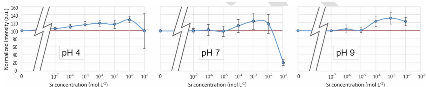
Fig. 5 Fluorescence intensity at \lambda_{\text{ex}} = 330 nm, \lambda_{\text{em}} = 510 nm of the PDMPO-Si system at various pH as a function of the concentration of Si in mol L -1 .
