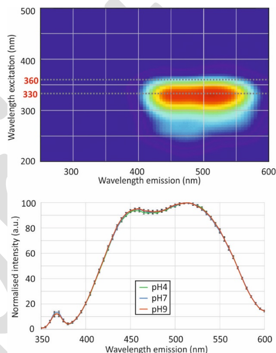
Fig. 3 PDMPO molecule fluorescence spectra. Top: bulk 3D spectra at pH 4 (Rayleigh diffusion was erased); bottom: normalized 2D spectras at \lambda_{\text{ex}} = 330 nm and pH 4, 7 and 9. Each spectra is the average of at least 10 measurements, vertical bars give the standard deviation.
