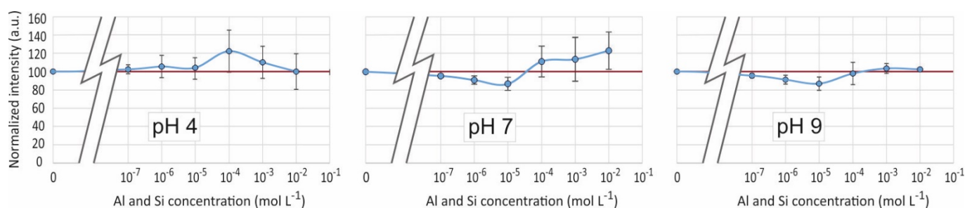
Fig. 10 Fluorescence intensities at \lambda_{\text{ex}} = 330 nm, \lambda_{\text{em}} = 510 nm of the PDMPO-Al-Si system at various pH as a function of the concentration of Al and Si in \text{mol L}^{-1} .
