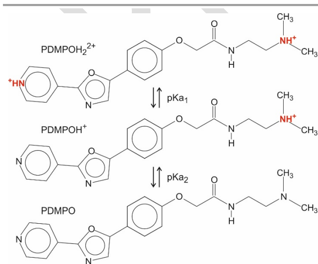
Scheme 1 Structure and protonation of PDMPO
