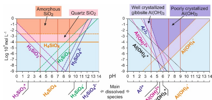
Fig. 6 Dissolved species concentration at equilibrium and precipitation domains in aqueous solution for Si (left) and Al (right) at 25°C. Calculation was done using the MINTEQA2 database values. 18 Plain lines: species at equilibrium with well crystallized minerals; dashed lines: species at equilibrium with poorly crystallized or amorphous minerals. Vertical red plain lines mark the studied pHs.
