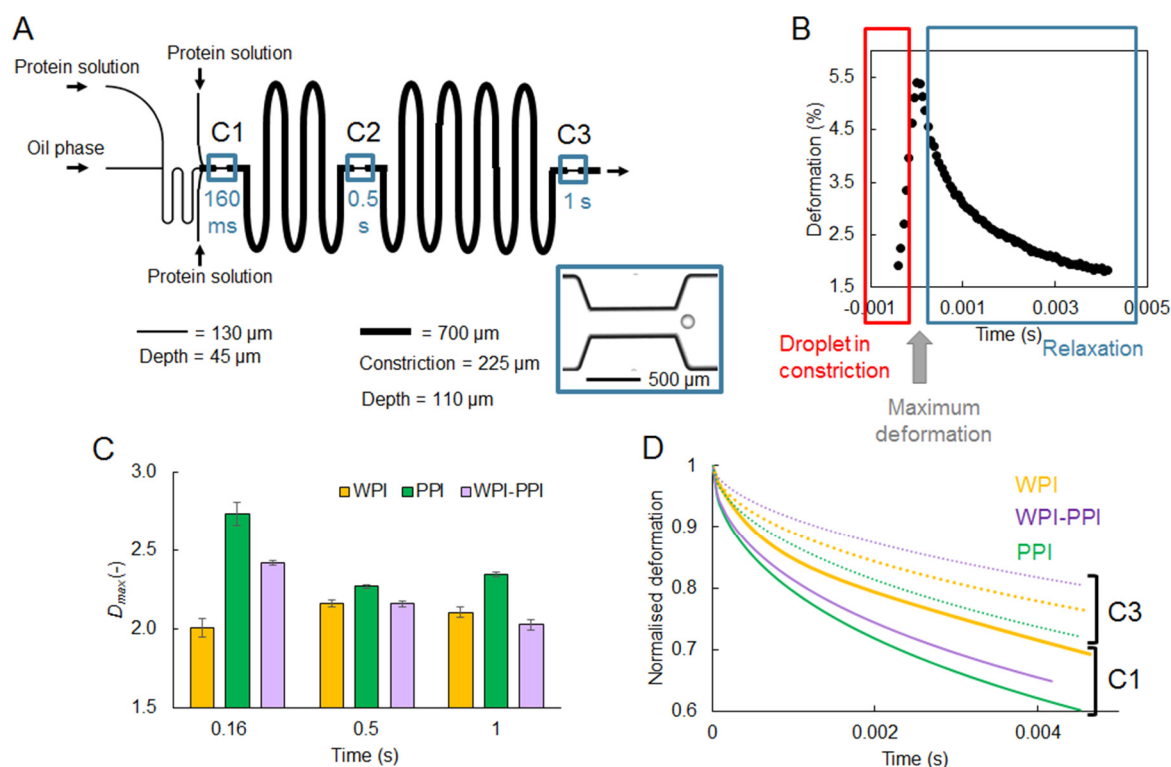
Figure 9. (A) Layout of the microfluidic rheology chip. The T-junction where droplets are formed (on the left) is the same as in the coalescence chip (Figure 7). The three constrictions (C1, C2, and C3) have a 70° angle. (B) Typical deformation pattern in time recorded by image analysis through passage of an emulsion droplet in a constriction. (C) Examples of maximum droplet deformations measured for droplets stabilized by different proteins (WPI, whey protein isolate; PPI, pea protein isolate; WPI-PPI, blend of both in 1:1 mass ratio), at the different constrictions C1, C2, and C3. (D) Examples of normalized relaxation curves for droplets stabilized by the same proteins, at constriction C1 (solid lines) or C3 (dotted lines). Reproduced from [89], under the CC BY license 4.0.
