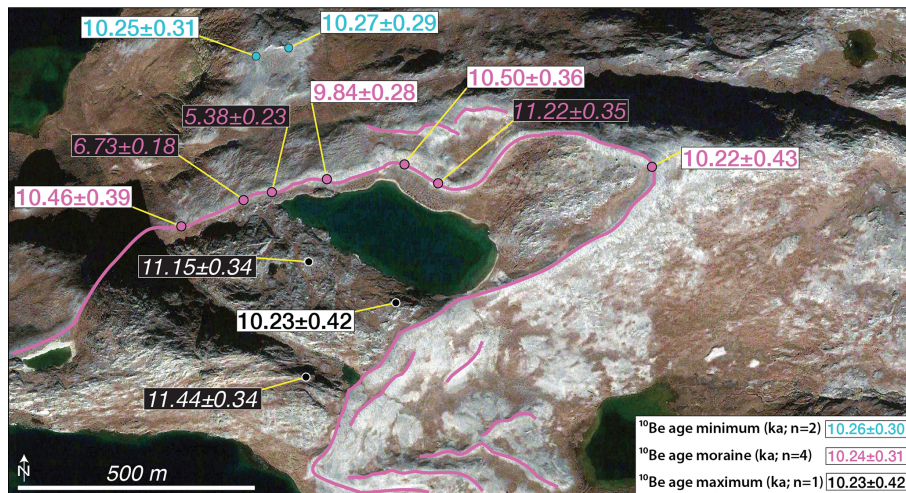
Figure 7. Kapisigdlit stade moraine located just west of KNS (Fig. 2). ^{10}\text{Be} ages (ka ± 1 SD) are from three morphostratigraphic groups: (1) outboard of the moraine (black text and symbols), (2) moraine boulders (pink text and symbols), and (3) inside the moraine (blue text and symbols). ^{10}\text{Be} ages that are considered outliers are in black boxes with italics. Map data: © Google Maps, Maxar Technologies.
