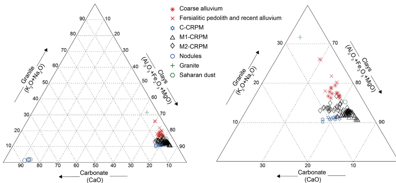
FIGURE 3 Geochemical ternary plot of XRF data obtained in bulk soil samples, carbonate nodules, dust and granite. The ternary plot on the left-hand side displays the samples within the full variation span; the right-hand side plot is a close-up of the sample distribution without the nodules (which have a CaO content >80\% ). The three end members have been chosen according to their correlations with the first two principal components after PCA. Sample colour codes refer to five different sample groups according to a cluster analysis: group 1 denotes the coarse alluvium ( n = 13 , samples from R and Q profiles), group 2 corresponds to the fersiallitic pedolith and recent alluvium ( n = 6 , samples T1–T6, and A1), group 3 to samples from the centre of Mima 1 ( n = 12 ), group 4 to the other samples of Mima 1 ( n = 64 ), and finally group 5 to samples from Mima 2 ( n = 23 ). Granite, Saharan dust and nodules are also displayed in the ternary plot, but they were not used in the cluster analysis
