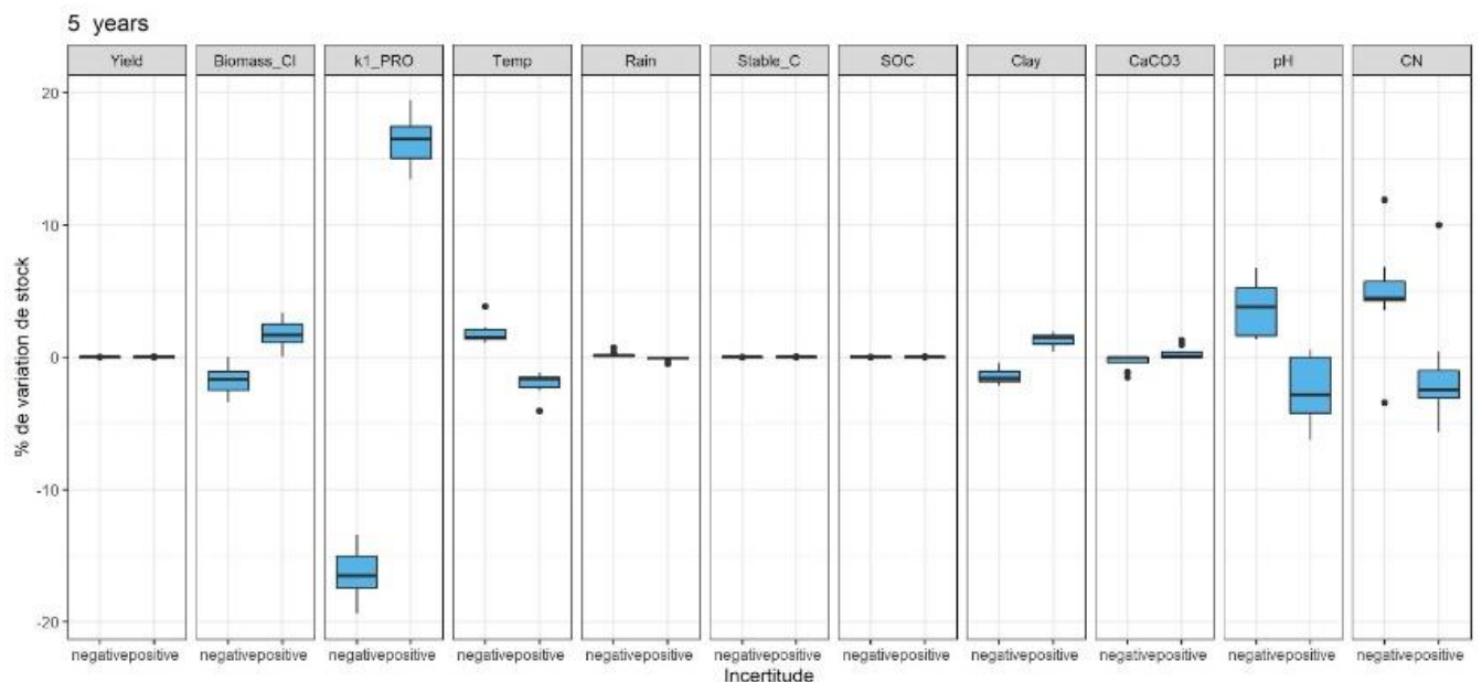
Figure 3 Results of Figure 3 expressed as % change in initial C stock. Sensitivity analysis of carbon sequestration after 5 years resulting from the application of carbon storing practices (I.C. and PROs, difference between the two practice scenarios).
