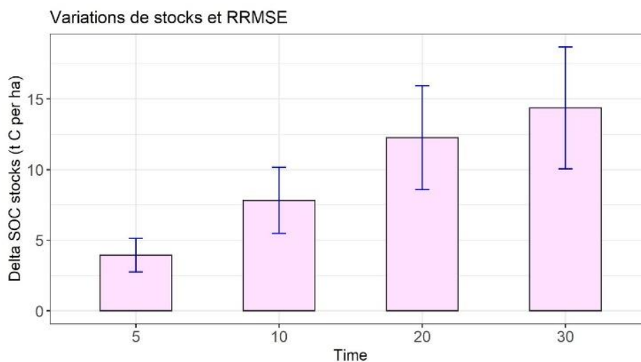
Figure 5: Median values of simulated stock changes (carbon storing systems vs. controls). The error bars correspond to the relative error of the model (RRMSE = 30%) at 5, 10, 20 and 30 years.
