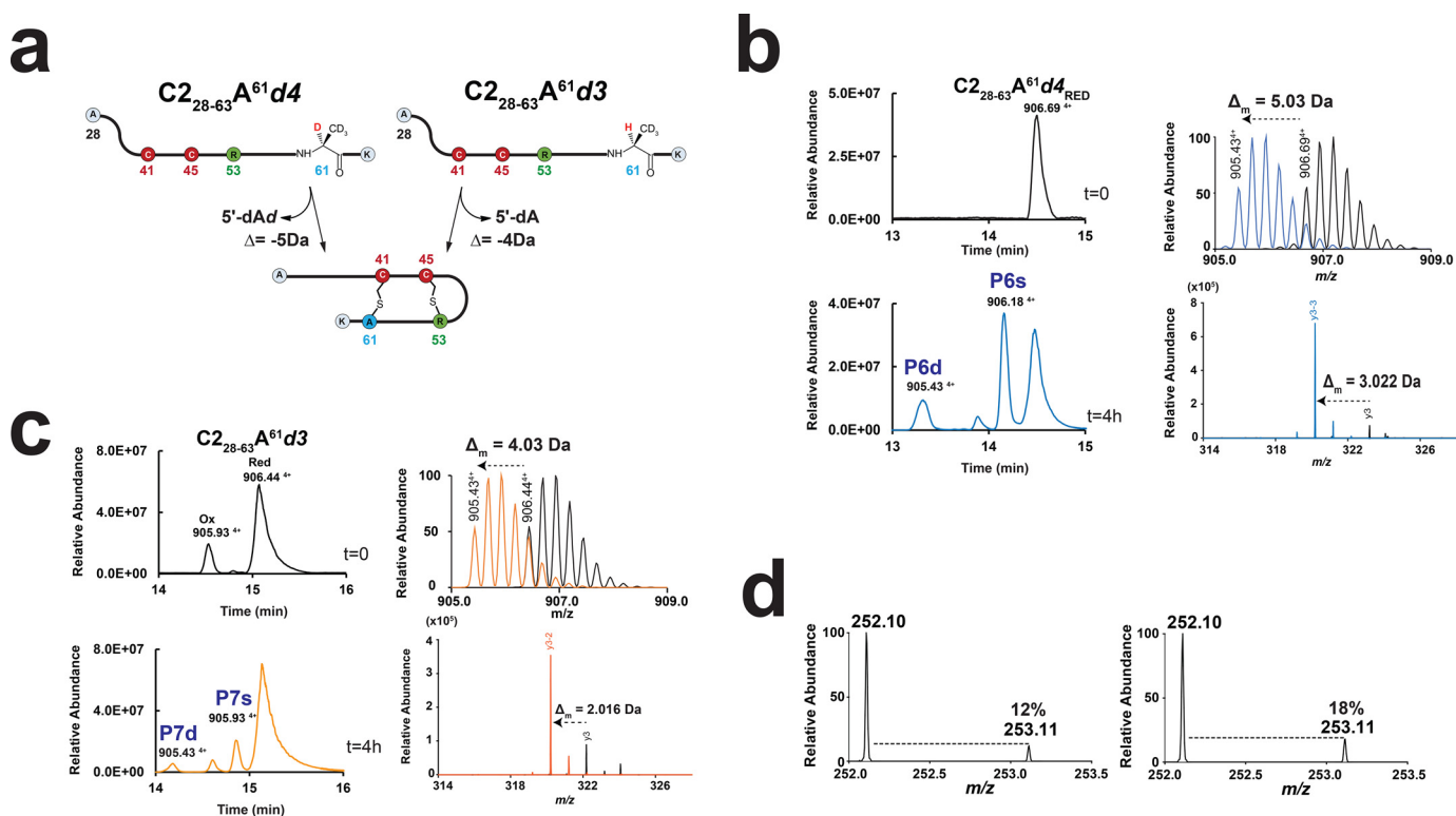
Figure 5. Activity of RumMC2 on the C_{228-63}A^{61}d3 and C_{228-63}A^{61}d4 deuterated peptides. a , sequence of the C_{228-63}A^{61}d4 and C_{228-63}A^{61}d3 peptides. The expected mass shift with the doubly bridged product ( i.e. -4 and -5 Da, respectively) is indicated. Only with the C_{228-63}A^{61}d4 peptide, production of 5' -dA, enriched with deuterium ( i.e. 5' -dAd), is expected. b , LC-MS analysis of C_{228-63}A^{61}d4 peptide before (upper left panel) and after 240 min of incubation with RumMC2 (lower left panel). Mass spectra of the substrate ( [M + 4H]^{4+} = 906.69 ) and the doubly bridged product ( [M + 4H]^{4+} = 905.43 ) are indicated (upper right panel). The relevant y_3 ion fragment originating from the product (blue trace; lower right panel) is superimposed with the y_3 ion fragment from the substrate (black trace; lower right panel). See Fig. S8, Fig. S9, Table S1 and Table S7 for full assignment. c , LC-MS analysis of C_{228-63}A^{61}d3 peptide before (upper left panel) and after (lower left panel) 240 min of incubation with RumMC2. Mass spectra of the substrate ( [M + 4H]^{4+} = 906.44 ) and the doubly bridged product ( [M + 4H]^{4+} = 905.43 ) are indicated (upper right panel). The relevant y_3 ion fragment originating from the product (blue trace; lower right panel) is superimposed with the y_3 ion fragment from the substrate (black trace; lower right panel). See Table S8 for full assignment. d , mass spectra of 5' -dA produced in the presence of the C_{228-63}A^{61}d3 (left panel) or C_{228-63}A^{61}d4 peptide (right panel). Percentage indicates isotopic distribution at m/z = 253 .
