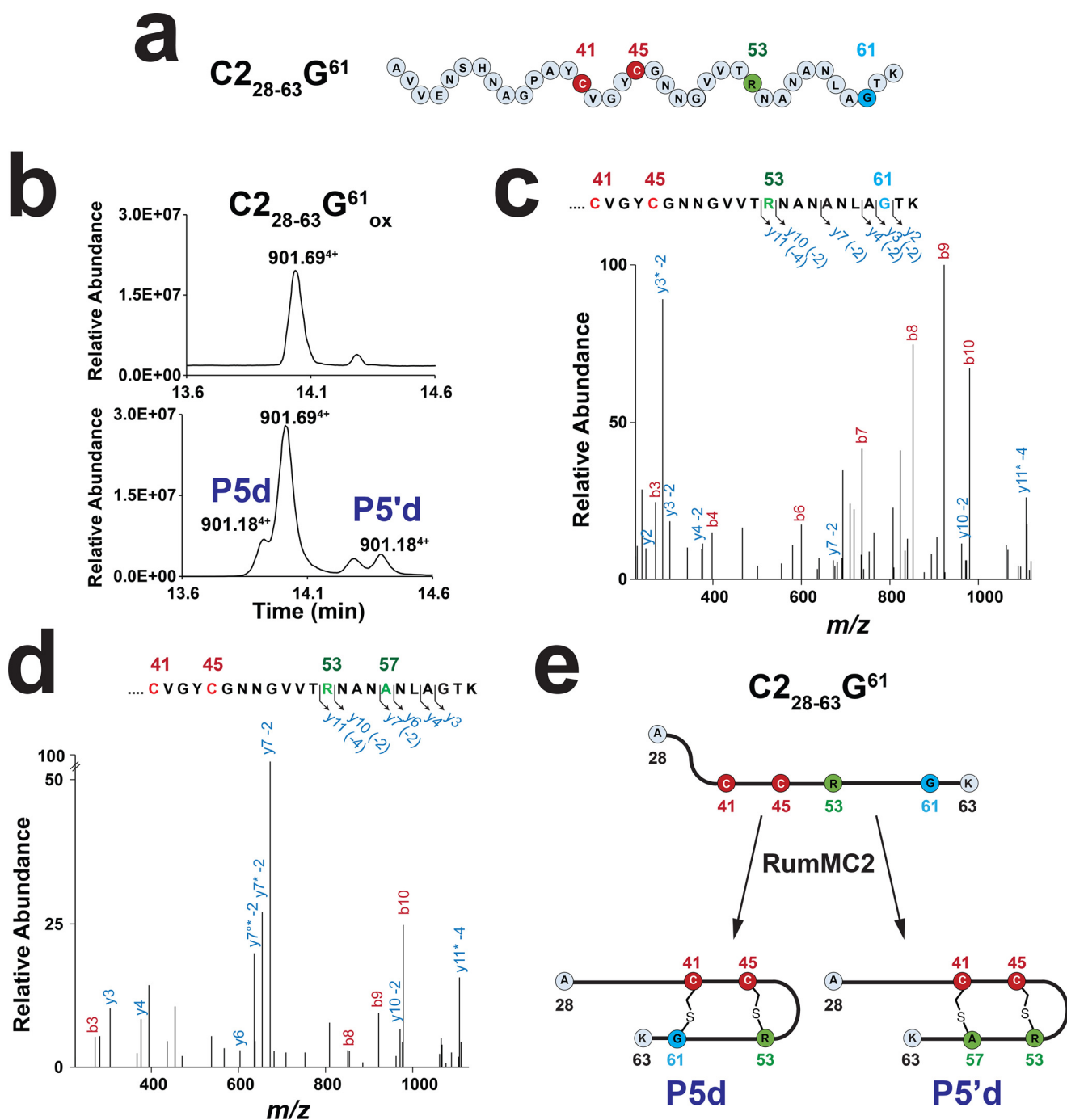
Figure 4. Activity of RumMC2 on a glycine-containing peptide (C 2 28-63 -G 61 ). a , sequence of the C 2 28-63 -G 61 peptide. Numbering refers to position of amino acid residues in C 2 . Amino acid residues involved in thioether bridges are indicated in red (cysteine) and green. The substituted residue is highlighted in blue. b , LC-MS analyses of the C 2 28-63 -G 61 peptide before (upper panel) and after (lower panel) 240 min of incubation with RumMC2. Two new species, P5d and P5'd, with a mass of [M + 4H] 4+ = 901.18 were produced. c , MS/MS analysis of P5d. Relevant ion fragments are indicated. As shown, the y 4 - 2 Da, y 3 - 2 Da, and y 2 ions allow to position the second thioether bridge on G 61 . Asterisk indicates loss of ammonia (-17.02 Da). See Table S1 and Table S6 for full assignment. d , MS/MS analysis of P5'd. Relevant ion fragments are indicated. As shown, the y 7 - 2 Da and y 6 ion fragments allow to position the second thioether bridge on Ala 57 . Asterisk indicates loss of ammonia (-17.02 Da). See Table S1 and Table S6. e , conversion of the C 2 28-63 -G 61 peptide into two doubly bridged peptides by RumMC2.
