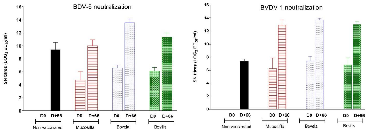
Figure 3. Mean neutralizing antibody titers (VNT) calculated by the Spearman-Kärber method and expressed in log 2 . Sera from D0 and D+66 of vaccinated (Mucosiffa in red, Bovela in blue, Bovilis in green) and unvaccinated (in dark) ewes were tested against the BVDV-1a NADL and the BDV-6 6390 strains for neutralization. Standard errors of the mean are indicated.
