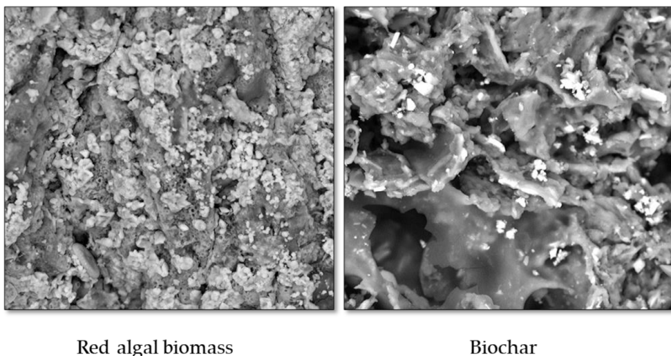
Figure 12. SEM image of red algal biomass and its biochar produced by pyrolysis at T = 450\text{ }^{\circ}\text{C} and \beta = 50\text{ }^{\circ}\text{C/min} .
