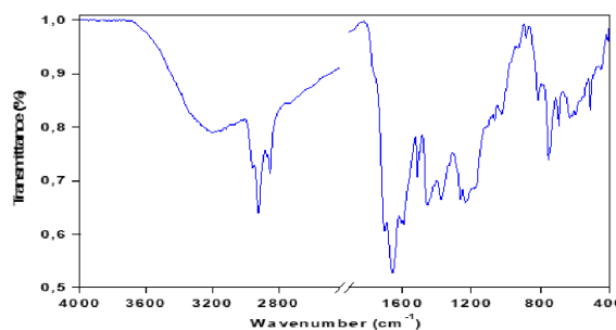
Figure 7. FTIR spectra of bio-oil produced by pyrolysis of red algal biomass ( T = 450\text{ }^{\circ}\text{C} and \beta = 10\text{ }^{\circ}\text{C}/\text{min} ).
