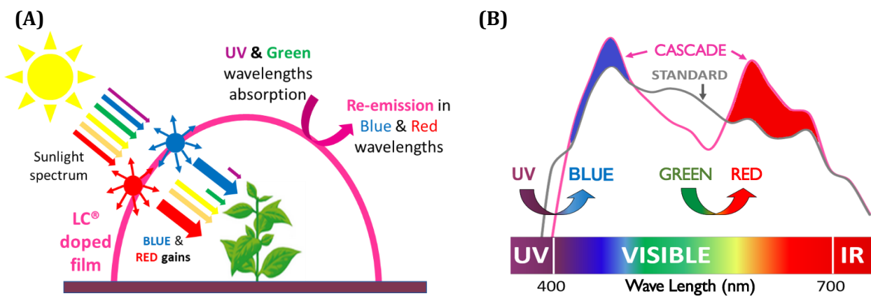
Figure 2. Illustration of the effect of the LC® technology on the solar spectrum.
