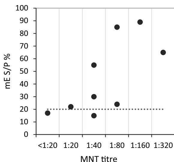
Fig. 2 Comparative analysis of serum for TBEV antibodies with microneutralization test (MNT) and modified indirect ELISA (mE). The dotted line indicates an S/P % value of 20 in mE. Of the MNT positive sera, 7 of 8 got S/P % values of \geq 20 with mE. One positive serum with an MNT titre of 1:40 got an S/P % value of 15, while one negative MNT serum got an S/P % value of 17
