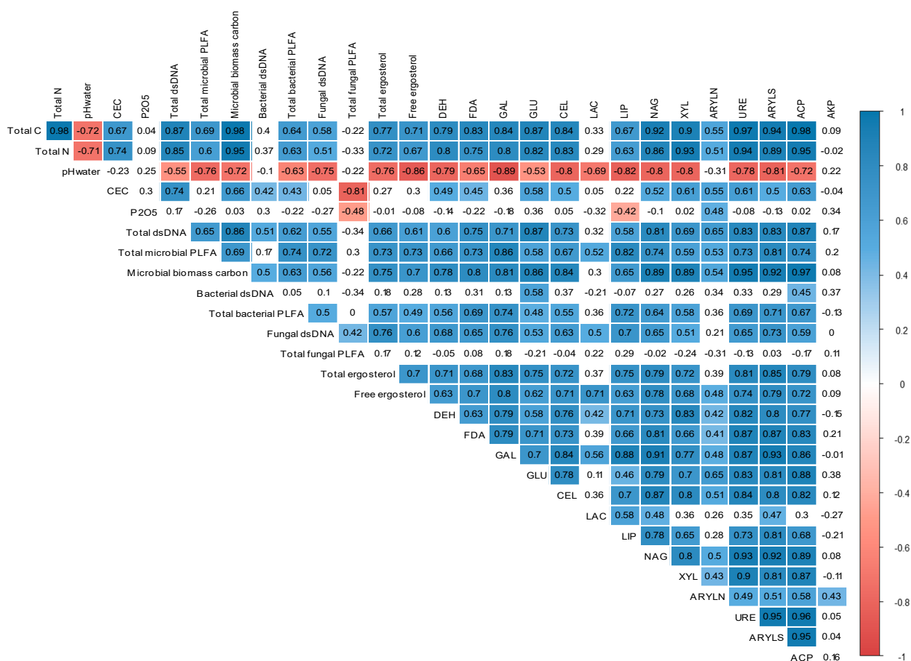
Figure 3. Correlation matrix between physicochemical parameters, microbial abundance, and enzyme activities. Red and blue color indicate statistically significant negative and positive correlations, respectively.
