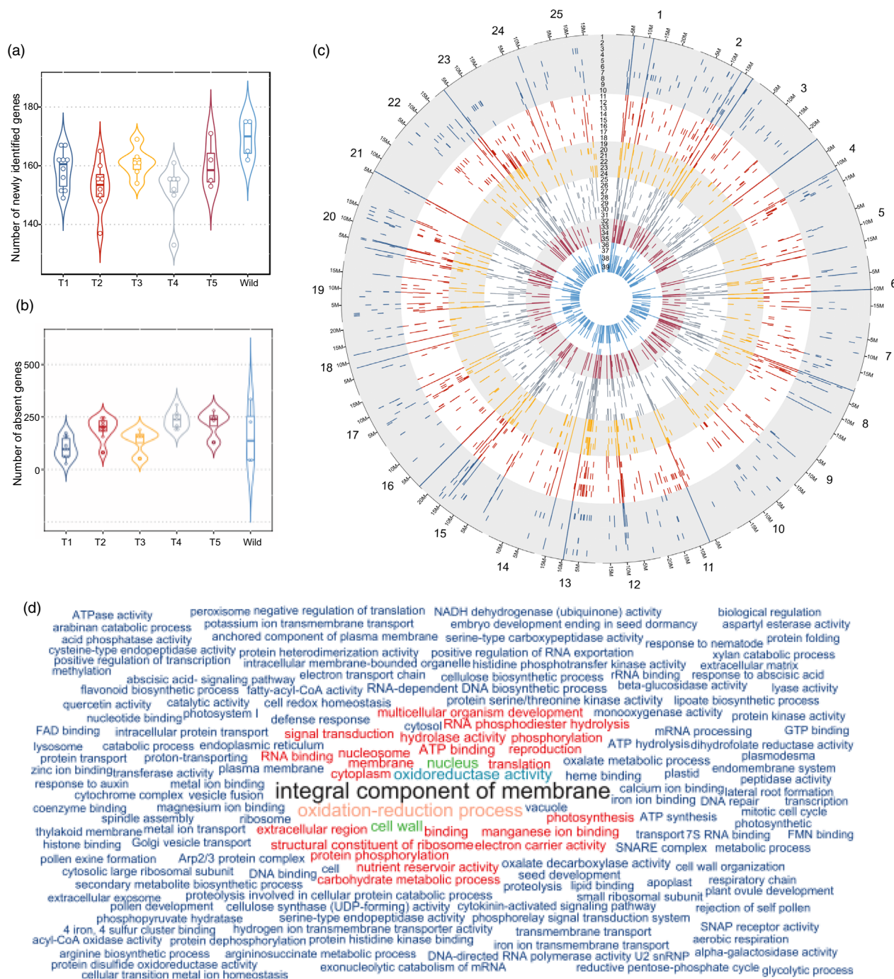
Figure 3 PAV of coding gene in L. albus . (a) Number of newly identified genes by phylogenetic group. (b) Number of absent genes by phylogenetic groups. (c) Positioning of absent genes in the 25 white lupin chromosomes in each 1 of the 39 accessions. Order of accessions from outer to inner track: 1-AMIGA, 2-FEODORA, 3-FIGARO, 4-ENERGY, 5-KIEV MUTANT, 6-HANSA, 7-P21525, 8-PRIMORSKY, 9-DIETA, 10-VOLODIA, 11-START, 12-N3507, 13-TOMBOWSKIJ, 14-KALINA, 15-SYR6258B, 16-LUCKY, 17-MURRINGO, 18-SHINFIELD, 19-ALB01, 20-LUXE, 21-ULYSSE, 22-MAGNUS, 23-CLOVIS, 24-ORUS, 25-NAHRQUELL, 26-GYUNLATANYA, 27-NEULAND, 28-NEUTRA, 29-BADAJAZ, 30-EGY6484B, 31-POUTIGANO, 32-P27174, 33-GERELTA, 34-DOGAN, 35-WADO, 36-GR38, 37-GRAECUS, 38-BATSI, and 39-GRC5262B. The accessions' colours reflect the six idiotypes. (d) Functional enrichment analysis of the variable genome. Graphical representation of enriched biological process (GOs). Size of the words and colours are proportional to their representativeness in the gene pool.
