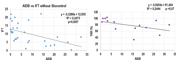
Figure 5: AIDB vs IFT without biocontrol (left) and AIDB vs YAR (%) (right). Yield Achievement Rate, as (Obtained yield / Expected Yield)*100 (right).
