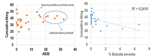
Figure 6: Organoleptic quality: AIDB vs Cumulative liking (left) and % of Botrytis severity (%) vs Cumulative liking in the young experimental wines
