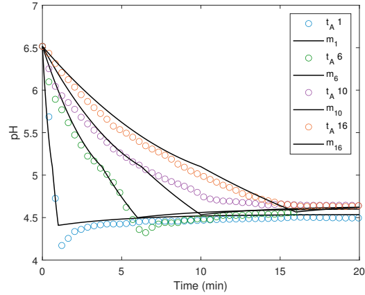
Fig. 6. Validation of the model. Data from (Hofland et al., 2003). Stirring rate 500 rpm, temperature 40°C
