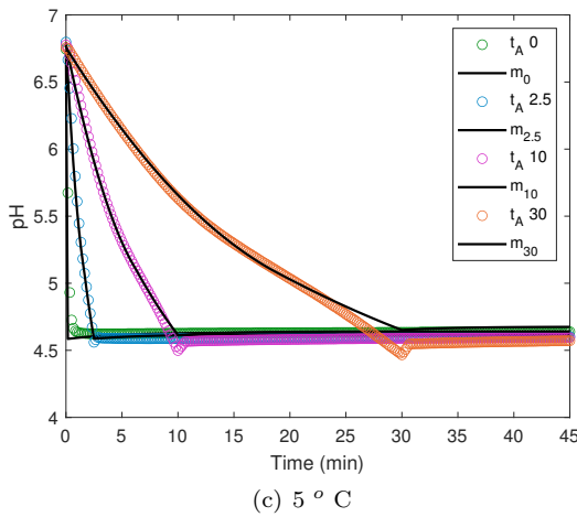
Fig. 5. Model outputs against experimental data. Dots represent experimental data, solid lines are model outputs for the different acidification times t_A .
