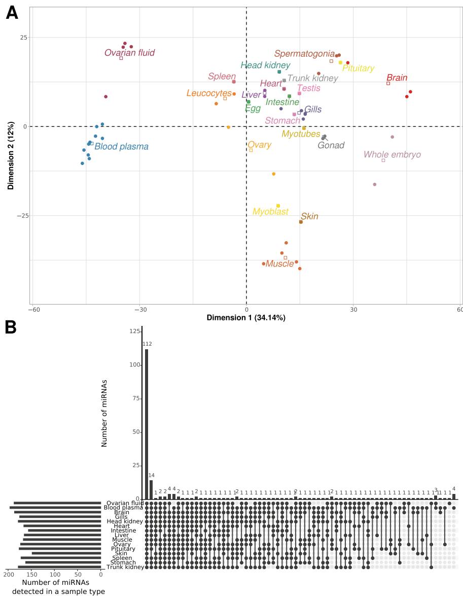
Fig. 4 Detection of blood plasma and ovarian fluid miRNAs in various organs and cell types. A PCA analysis of normalized RPM counts supplied by ProSt using all samples ( N=52 ). PCA was centered but not scaled. Corresponding data are available in additional file 4. B The number of circulating miRNAs detected in all possible combinations of analyzed libraries is displayed. Libraries in which miRNAs were detected are indicated by a black dot. miRNAs were considered present in an organ or a fluid if their normalized abundance exceeded 10 RPM, on average, for each type of sample. The analysis was limited to the two biological fluids (blood plasma and ovarian fluid) and a subset of 13 different female organs displayed in Fig. 3
