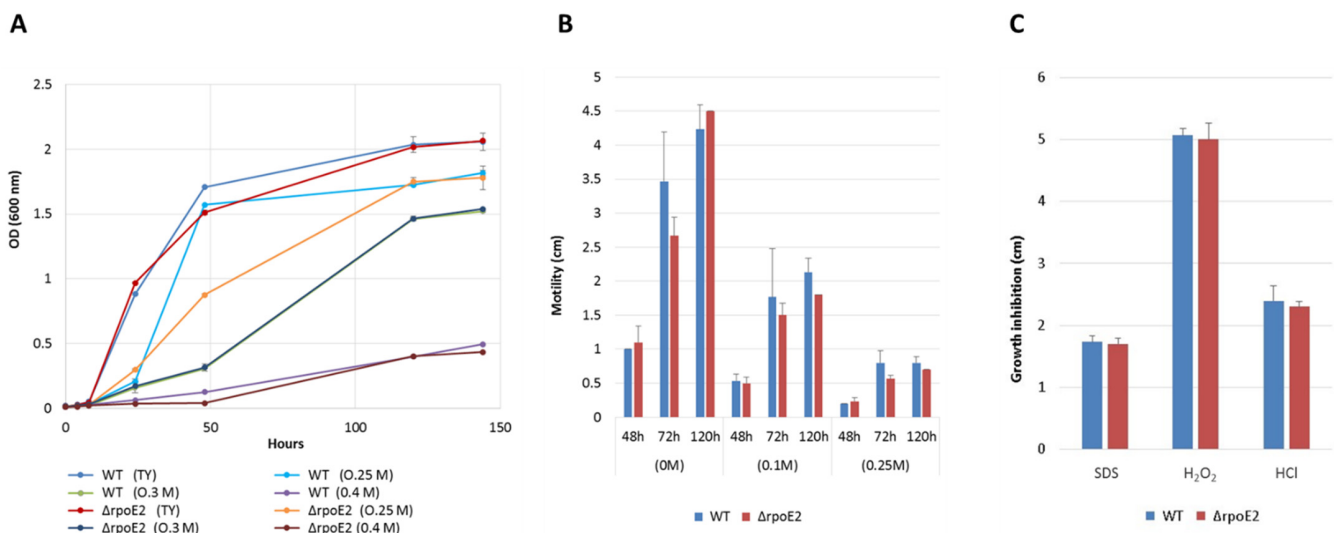
Figure 2. Effect of the rpoE2 mutation on stress tolerance and motility of LMR001. Ensifer aridi LMR001 (WT) and the LMR001 rpoE2 deletion mutant ( \Delta rpoE2 ) growths were compared in liquid TY medium complemented with 0, 0.1, 0.25, 0.3, or 0.4 M of NaCl (A). Their motility was assessed in semi-solid TY complemented with salt at 0, 0.1, or 0.25 M by measurement of the diameter of the swimming colonies after 2, 3, or 5 days of incubation (B). Finally, the diameters of the growth inhibition zones were compared for the two strains inoculated in top agar plates, to the center of which patches imbued with 5 \mu L of SDS (10% w/v ), H 2 O 2 (5.5 M), or HCl (2 M) were placed (C).
