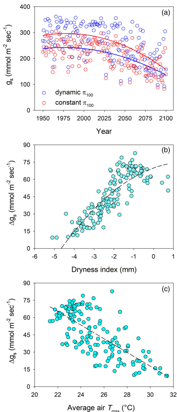
Figure 6. SurEau long-term model output using Bordeaux RCP8.5 simulation data for the years 1950–2100.
