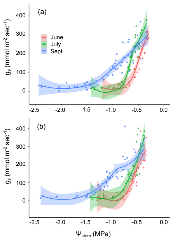
Figure 3. Stomatal conductance ( g_s ) response to stem water potential ( \Psi_{\text{stem}} ) during the three different drought experiments (in June, July, and September).
