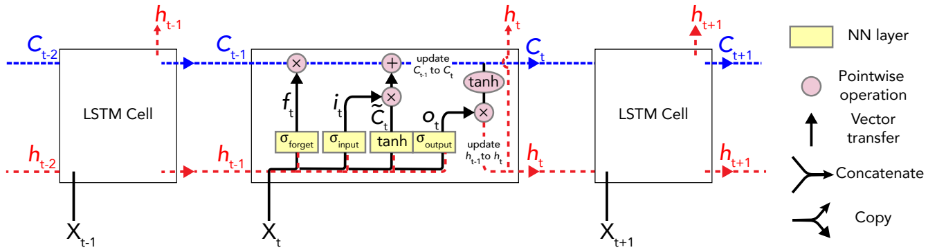
Figure 7. Time unfolded schematic representation of data processing through successive LSTM units. X_t is the input of time step t . h_t is the hidden state (dashed red line). C_t represents the cell state (dashed blue line). \sigma and \tanh are activation functions. NN stands for neural network. The figure is adapted from Chollet and Allaire (2018) and Olah (2015).
