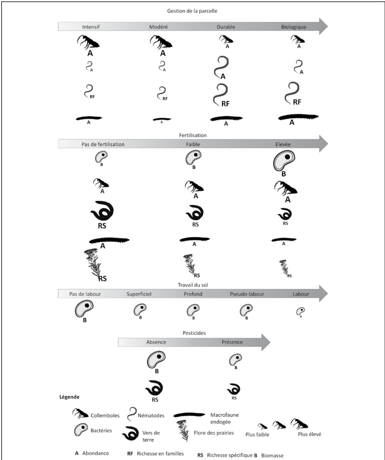
Figure 2 : Effect of management type, fertilization level, tillage and pesticide use on microorganisms, soil fauna and grassland flora (only taxa with significant differences between modalities are shown, based on Cluzeau et al. (2012) and Perronne et al. (2019)).
