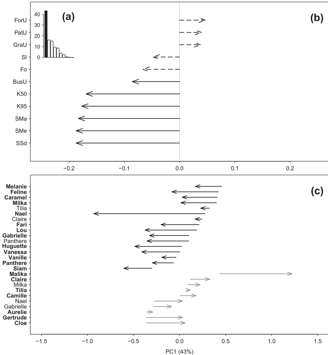
Figure 1. Principal component analysis performed to identify the effect of drive hunts on female red deer movement patterns in the NHWR of La Petite Pierre, France, 2004–2018. (a) Eigenvalues histogram displaying the amount of variation accounted for by each principal component. (b) Representation of the 11 movement variables' vectors along the first axis (black vertical bar in the histogram of eigenvalues). Vectors indicate the intensity and direction of each movement variable to the overall distribution of the hunting events. Solid arrows correspond to the variables that are significantly correlated with the first axis. The movement metrics are those described in Table 1. (c) Non-recentred drive hunt effect vectors ( n = 26 hunted animals) in the space defined by the spatial descriptors, along the first PCA axis. The basis of the vector corresponds to the score of the animal before the drive hunt and the top of the vector corresponds to the score of the animal after the drive hunt. Vectors indicate the intensity of the drive hunt effect and the variables that have changed the most in response to the drive hunt. Black arrows correspond to individuals characterized after the hunt by larger spatial descriptors and grey arrows correspond to individuals with the opposite characteristics. The individuals identified in bold have been located within a hunting area at the time of the drive hunt only once during a given hunting season.
