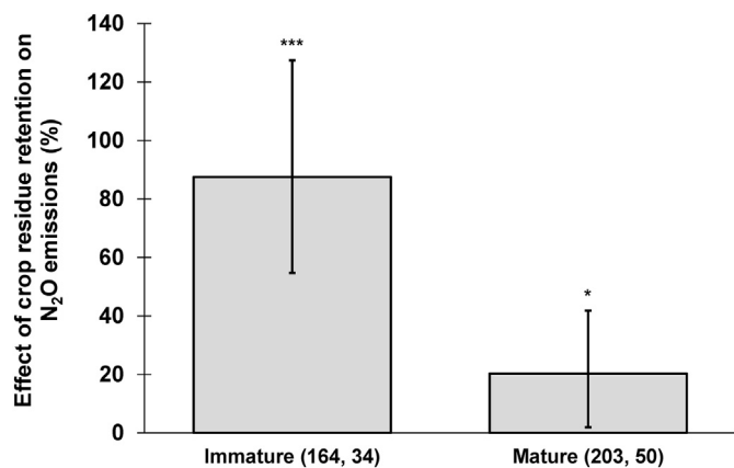
Fig. 4. Relative increase in field N 2 O emission (mean ± 95% CIs) with crop residue incorporation, as affected by residue maturity class. The number of observations and studies are shown in parentheses. See section 2.1.3. for a detailed description of the maturity criteria.
