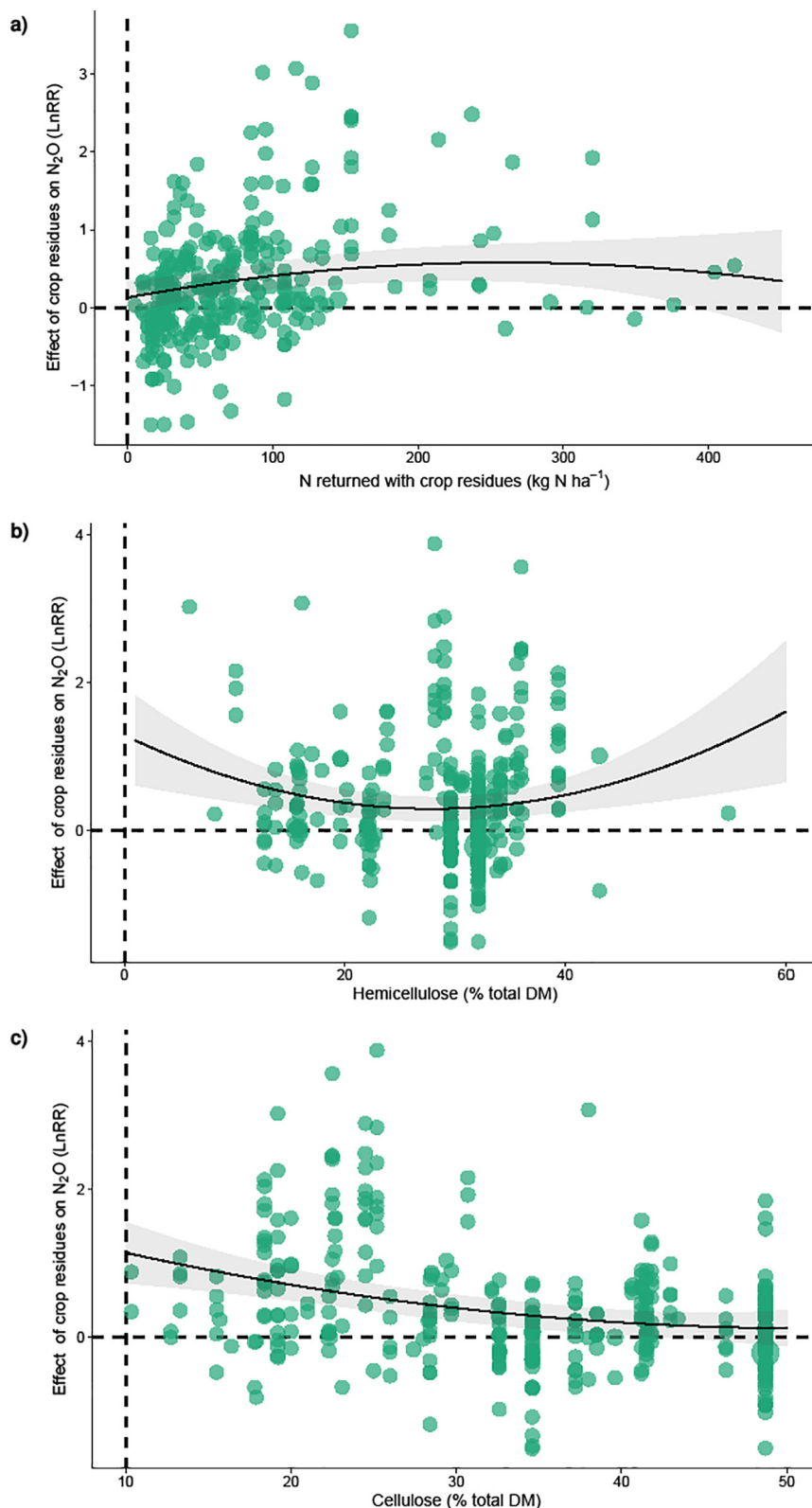
Fig. 2. Meta-analytic scatterplots of important factors controlling the effect of crop residue retention on N_2O emissions (identified by the random-meta-forest approach); a) N returned with crop residues ( kg\ N\ ha^{-1}\ yr^{-1} ), b) residue hemicellulose concentration (% DM), and c) residue cellulose concentration (% DM).
