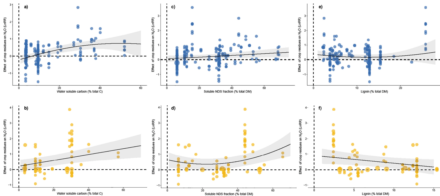
Fig. 3. Meta-analytic scatterplots of important factors controlling the effect of crop residue retention on \text{N}_2\text{O} emissions (identified by the random-meta-forest approach) and influenced by N fertilizer addition: Water soluble carbon (% total C), soluble NDS fraction (% DM), and lignin (% DM). Graphs in the top row (blue; a, c, e) show results for studies without N fertilizer application; the bottom row (yellow; b, d, f) shows results for studies with N fertilizer application. Note that the scale of the horizontal axes for lignin are different for fertilized and unfertilized meta-regressions. (For interpretation of the references to colour in this figure legend, the reader is referred to the web version of this article.)
