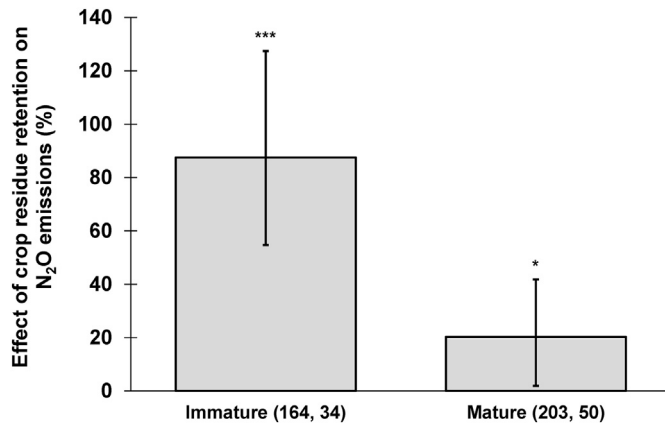
Fig. 4. Relative increase in field N_2O emission (mean \pm 95% CIs) with crop residue incorporation, as affected by residue maturity class. The number of observations and studies are shown in parentheses. See section 2.1.3. for a detailed description of the maturity criteria.
